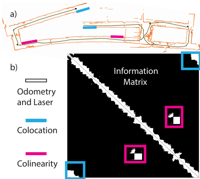
Figure 5: Example map (a) with corrections and resulting information matrix (b). The white band diagonal represents the correlations from the initial factor graph G_0 . The colored lines on the map show the human correction input: colocation (blue) and collinear (magenta).. The constraints correspond to the blue and magenta off-diagonal entries in the information matrix.
